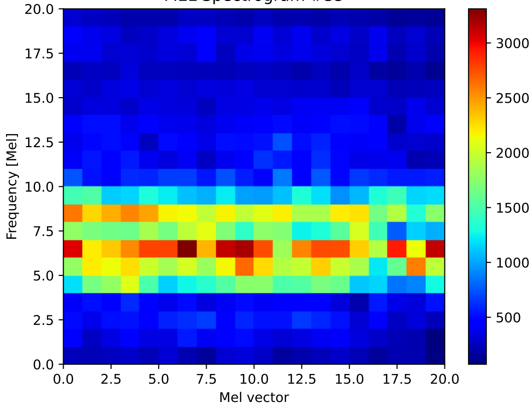
MEL Spectrogram #35
